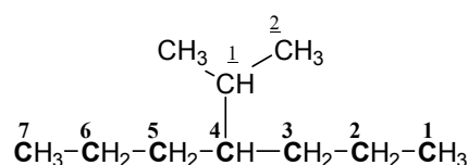
4-Isopropyl heptane or 4-(1-methyl ethyl) heptane
