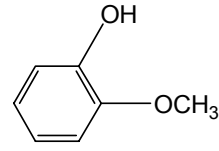
o-Hydroxy anisole [Guaiacol]
