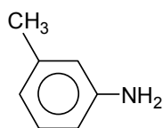
m-Toluidine
