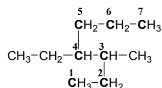
4-Ethyl-3-methyl heptane
