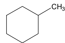
Methyl cyclohexane
