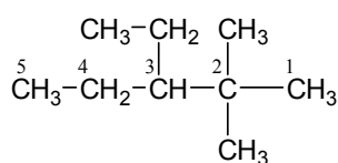
3-Ethyl-2,2-dimethyl pentane
