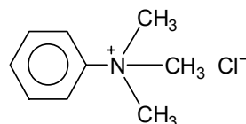
N,N,N-Trimethyl anilinium chloride
