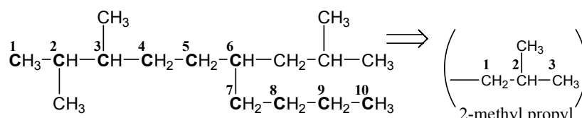
6-Isobutyl-2,3-dimethyl decane or 2,3-Dimethyl-6-(2-methyl propyl) decane
