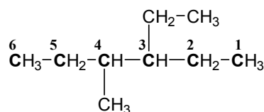
3-Ethyl-4-methyl hexane
