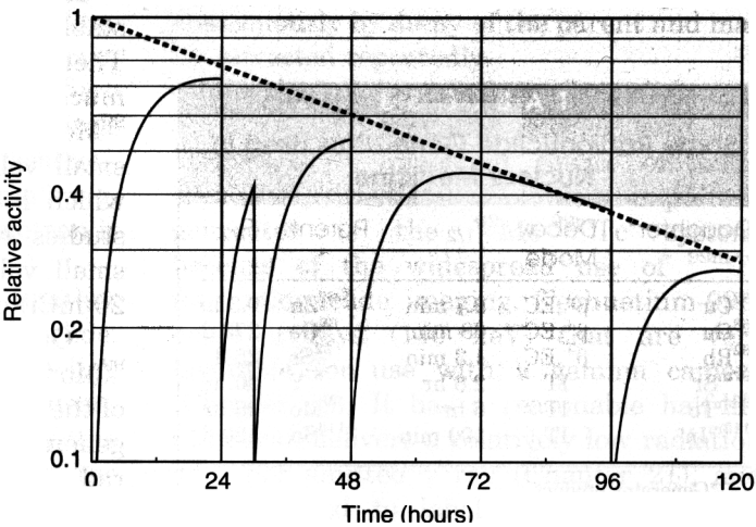
Figure 5-7. Buildup and decay of a ^{99\text{m}}\text{Tc} generator eluted at 24, 30, 48, and 96 hours.
