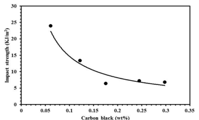
Fig-6: The effects of carbon black content on the impact strength [processing temperature 180°C: processing time 7 min: fiber content 3.07%].
