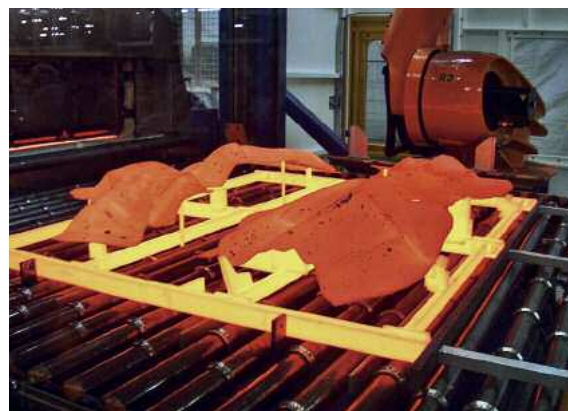
Sheet plate components pre-heated to 950°C [© Volkswagen AG, Presswerk Kassel]
