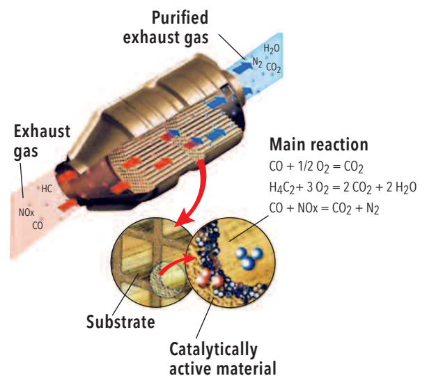
Functionality of a car exhaust catalyst [© Umicore AG & Co. KG]
