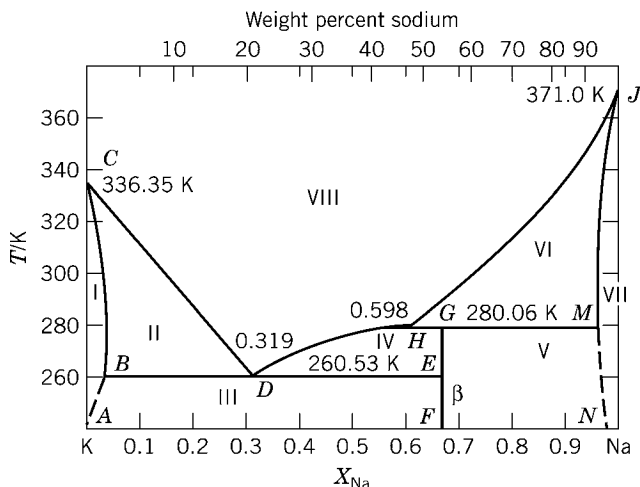
Figure 13.6. The phase diagram at constant pressure of the system Na-K. With permission, from R. Hultgren, D. T. Hawkins, M. Gleiser, and K. K. Kelley, Selected Values of Thermodynamic Properties of Binary Alloys , American Society of Metals, Metals Park, OH, 1973, p. 1057.
