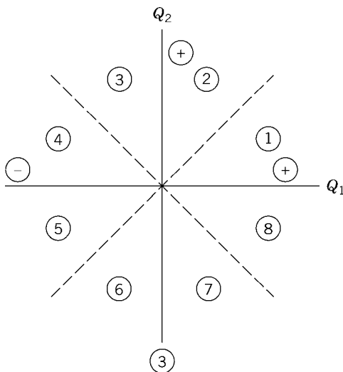
Figure 6.11. Sketch of the Q_2 – Q_1 coordinate system for possible Carnot cycles.
