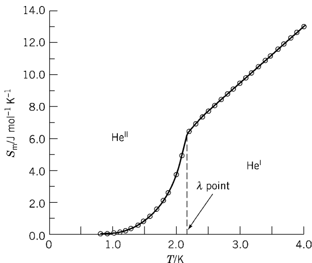
Figure 11.6. Entropy of liquid ^4\text{He} under its equilibrium vapor pressure. Data below 1.90 K from H. C. Kramers, J. D. Wasscher, and C. J. Gorter, Physica 18 , 329 (1952). Data from 1.90 K to 4.00 K from R. W. Hill and O. V. Lounasmaa, Phil. Mag. Ser. 8 , 2 , 143 (1957).
