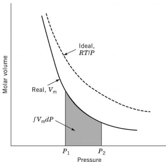
Figure 10.6. Comparison of molar volume–pressure isotherms for a possible real gas and an ideal gas.
