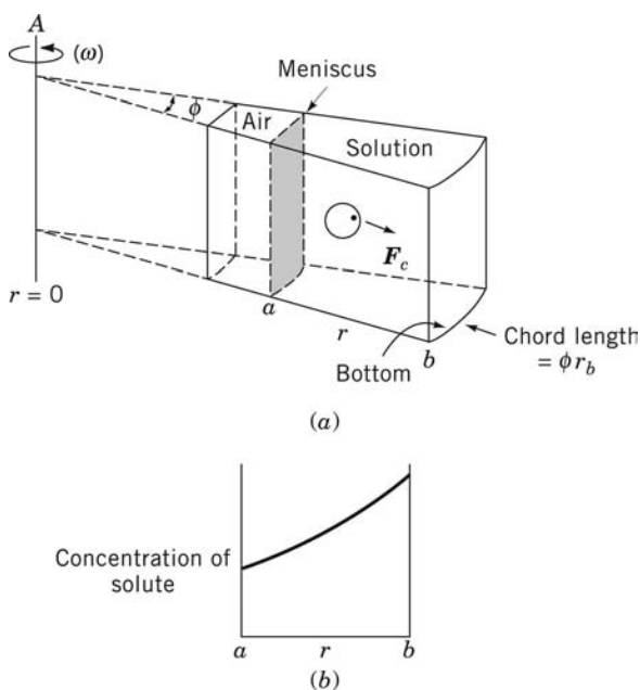
Figure 21.2. (a) Schematic diagram of a sedimentation apparatus for determination of molecular mass of a solute molecule. The sector-shaped container is actually mounted in a rotor that spins about an axis of rotation A at an angular velocity \omega . The centrifugal field, \mathbf{F}_c at any point is directed along the axis r in the direction of increasing r . At any position r , the chord length is \phi r , which increases with increasing r . The position of the liquid meniscus is indicated by a . (b) Concentration distribution of solute in cell at sedimentation equilibrium.
