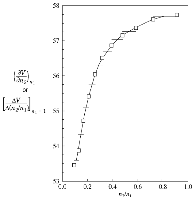
Figure 18.3. Graphical differentiation to obtain V_{m2} in ethanol–water solution compared with derivative of quartic fit of V as function of n_2/n_1 and numeric differentiation. The solid curve represents the result of differentiation of a fitted quartic polynomial of V as a function of n_2/n_1 . The squares represent the results of a numeric differentiation. The horizontal lines represent a graphical differentiation.
