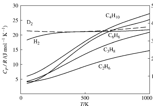
Figure 4.2. Variation of heat capacity with temperature as calculated from the equations of Frenkel et al. [4]. The differences observed between isotopic species and the way heat capacity depends on molecular size and structure can be described thermodynamically, but they must be explained by the methods of quantum-statistical thermodynamics. The right-hand scale is for H_2 and D_2 ; the left-hand scale is for the other compounds.
