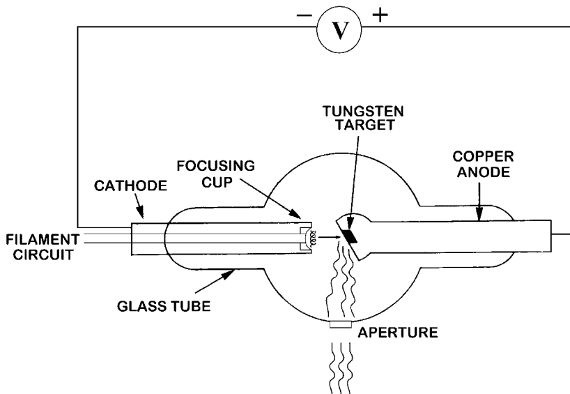
Fig. 15-2 Major components of a stationary anode x-ray tube.
