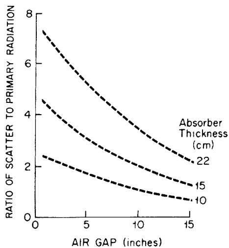
Fig. 15-21 Ratio of scatter to primary radiation reaching the x-ray film for various air gaps and patient thickness.
