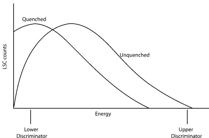
Fig. 12-16 Effect of sample quench in liquid scintillation counting is to lower the number of counts observed in a set window.
