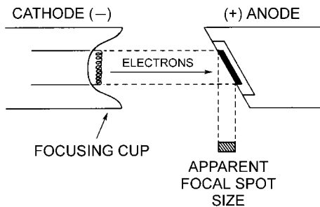
Fig. 15-5 Use of a focusing cup to achieve a thin electron beam and an angled anode to achieve a small apparent focal spot.
