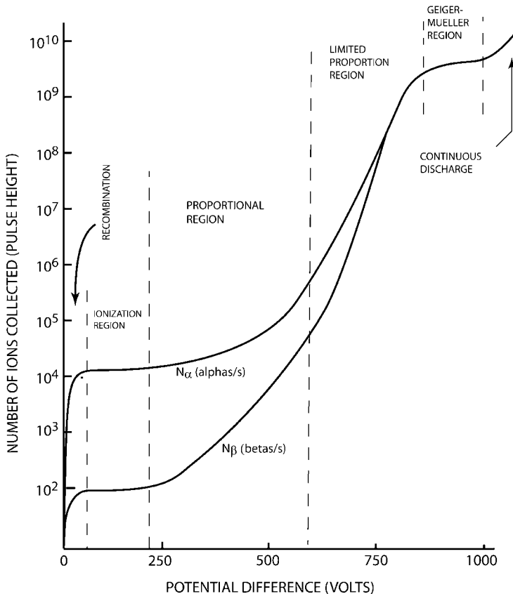
Fig. 12-2 Ionization rates for constant source strengths of a beta emitter and an alpha emitter in a gas-filled detector operated in different voltage ranges.
