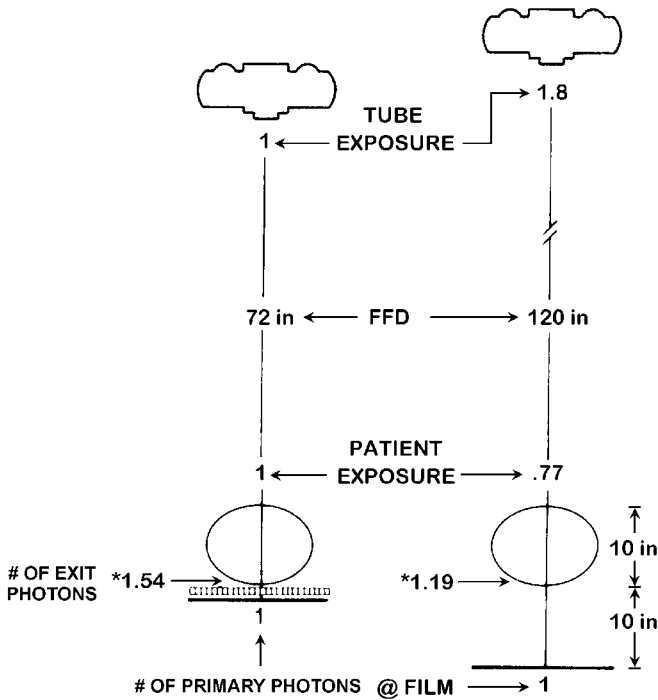
Fig. 15-22 Comparison of the grid technique and the air-gap technique for chest radiography.
