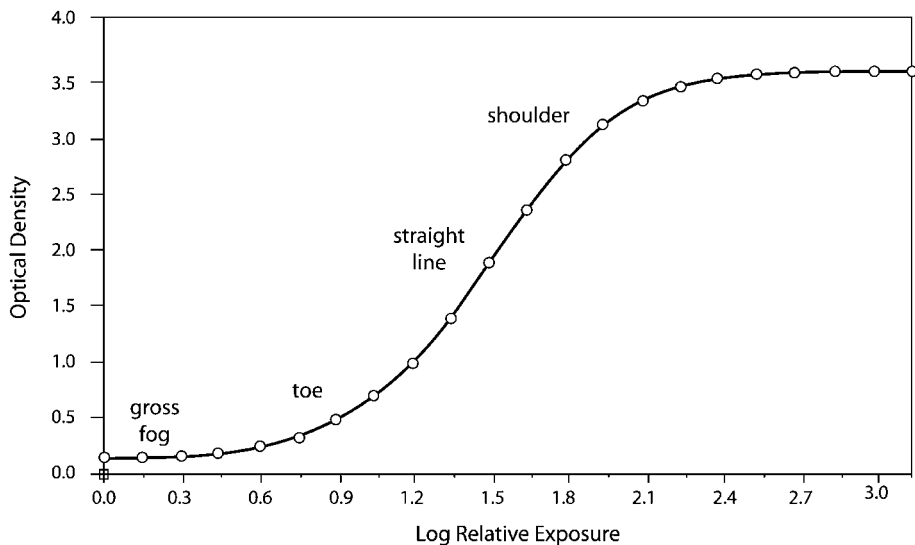
Fig. 15-26 Typical H and D (or characteristic) curve of optical density produced in x-ray film by varying amounts of x-ray exposure and its four principal regions.
