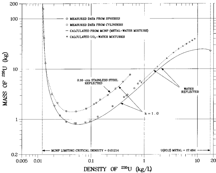
Fig. 11-5 Critical masses of spherical shapes of 93.2% ^{235}\text{U} in homogeneous water-moderated solution as function of ^{235}\text{U} density and reflection by thick water and stainless steel. (Adapted from Criticality Safety Guide with permission.)
