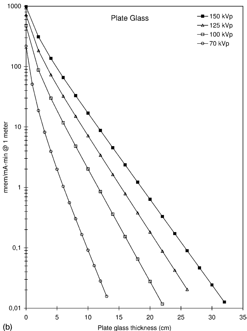
Fig. 15-31 Dose equivalent rate per mA min at 1 m for x-rays generated at various kVp values after transmission through thicknesses of (a) gypsum and (b) plate glass.
