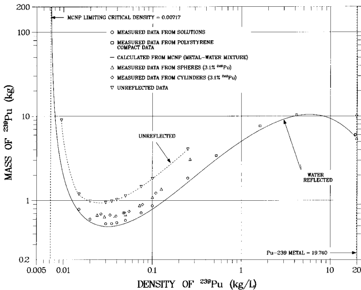
Fig. 11-6 Critical masses of spherical shapes of ^{239}\text{Pu} in homogeneous water-moderated solution as function of ^{239}\text{Pu} density with and without water reflection. (Adapted from Criticality Safety Guide with permission.)
