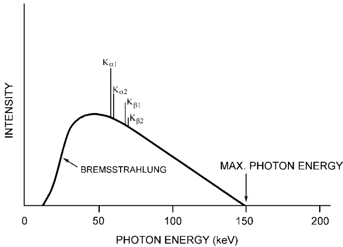
Fig. 15-3 Continuous spectrum of x-ray energies with E_{\max} corresponding to a maximum x-ray energy of 150 keV across the x-ray tube.
