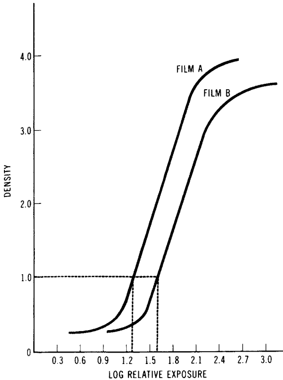
Fig. 15-27 Speed of a film is the reciprocal of the exposure, in roentgens, needed to produce a density of 1.0. Film A is faster than film B.
