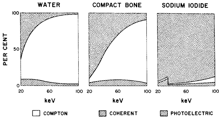
Fig. 15-18 Percent of coherent, photoelectric, and Compton reactions in water, compact bone, and sodium iodide. (Courtesy of Christensen, with permission.)
