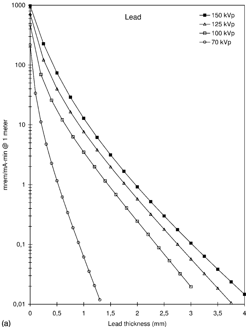
Fig. 15-30 Dose equivalent rate per mA min at 1 m for x-rays generated at various kVp values after transmission through thicknesses of (a) lead and (b) steel.
