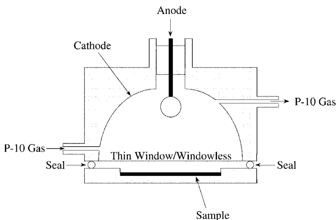
Fig. 12-17 A 2\pi proportional counter with a window; if used without a window in either 2\pi or 4\pi geometry, it is necessary to provide a mechanism to reseal the chamber after samples are inserted and to provide rapid flushing with the counting gas to replace any outside air.
