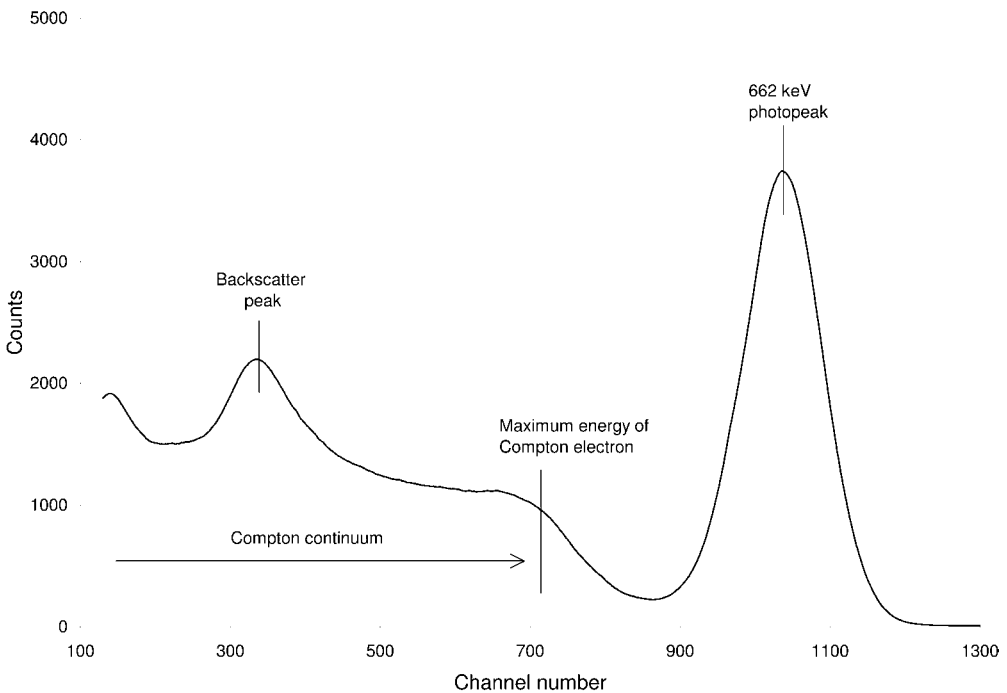
Fig. 12-6 Gamma ray spectrum obtained with a sodium iodide crystal exposed to 662 keV gamma rays of ^{137}\text{Cs} .
