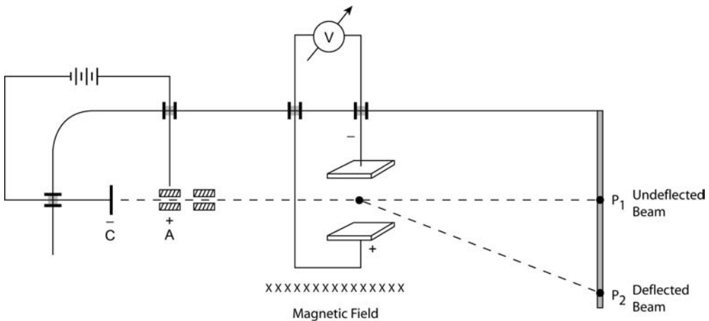
Fig. 2-4 J. J. Thomson's apparatus for measuring e/m of cathode rays by establishing the electric field required to exactly cancel the deflection (shown by a scale glued onto the end of the tube) induced by the magnetic force field.
