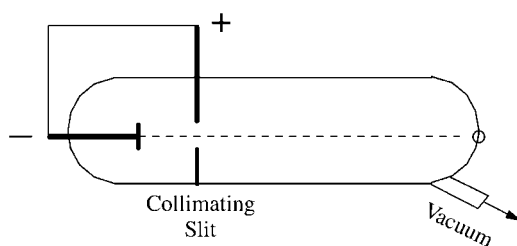
Fig. 2-1 Cathode-ray tube.
