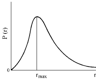
Fig. 2-30 Plot of the probability of finding an electron in hydrogen versus r , the distance from the nucleus. Note that r_{\text{max}} corresponds to the first Bohr radius shown in Figure 2-31.
