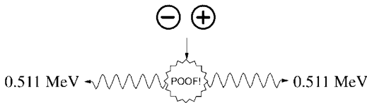
Fig. 3-8 Annihilation of a positron and a negatron, which converts the electron masses to electromagnetic radiation.
