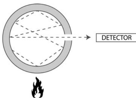
Fig. 2-8 Blackbody “cavity” with an external heat source.
