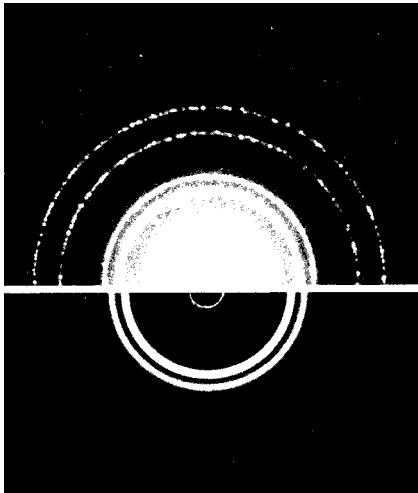
Fig. 2-27 Diffraction pattern produced by 600 eV electrons (top) and x-rays of 0.71 Å (bottom).
