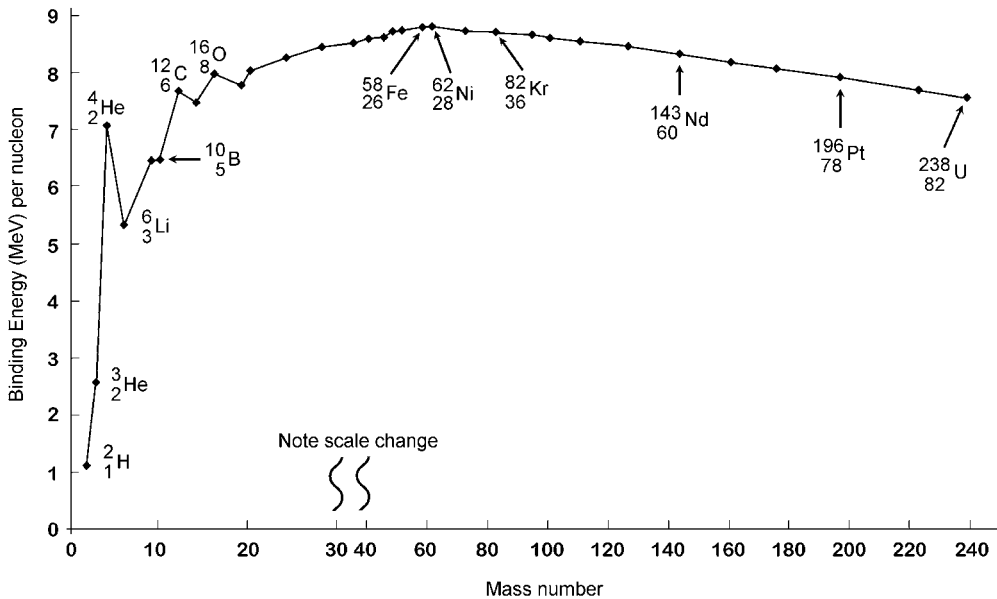
Fig. 1-3 Curve of binding energy per nucleon versus atomic mass number (plotted from data in Appendix B).
