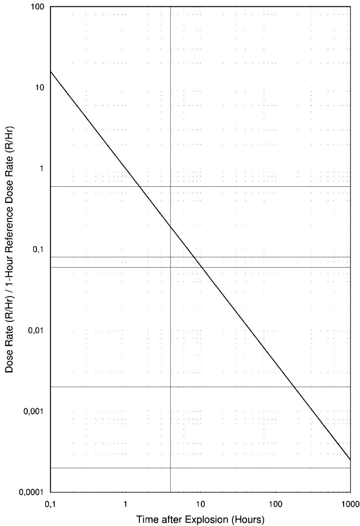
Fig. 11-3 Decrease of dose rate from fission products with time.
