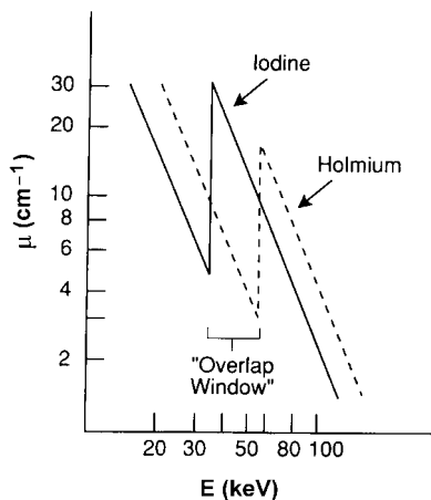
Fig. 15-17 Attenuation of photons by iodine and holmium in which the transmission of holmium enhances transmission of x-ray photons below 55.6 keV and absorbs those above it, while attenuation in iodine produces an “overlap window” of high contrast. (Adapted from Christensen, with permission.)
