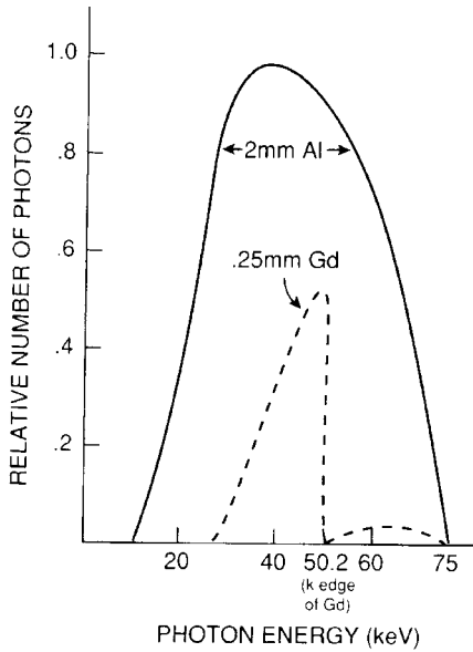
Fig. 15-16 Effect of a gadolinium filter on the bremsstrahlung spectrum of a 75 kVp x-ray beam with 2 mm aluminum filtration. (Courtesy of Christensen, with permission.)
