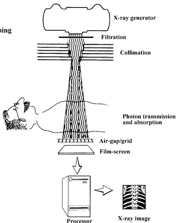
Fig. 15-1 Four major components of an x-ray system.
