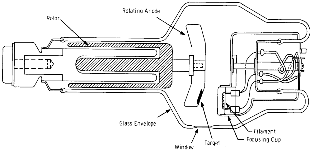
Fig. 15-9 Principal parts of a modern rotating-anode x-ray tube. (Courtesy of Bushong, with permission.)
