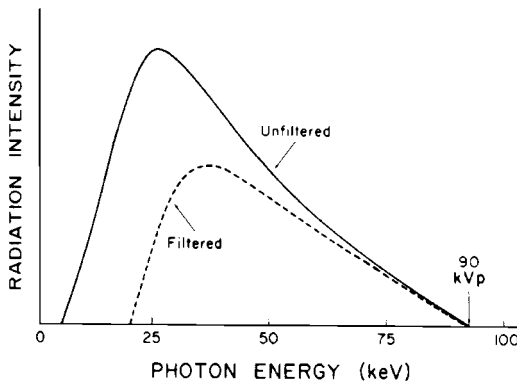
Fig. 15-14 Effect of filtration on average energy and intensity of a continuous x-ray spectrum produced by 90 kVp electrons on a tungsten target.
