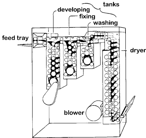
Fig. 15-25 Major components of an automatic film processor. (Adapted from Bushong (2004), with permission.)
