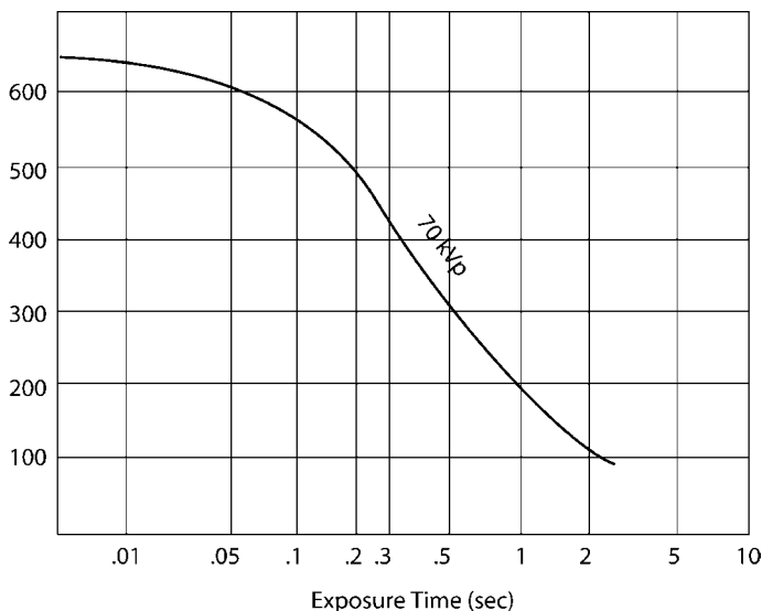
Fig. 15-10 Theoretical tube rating for an x-ray tube operated at 70 kVp.
