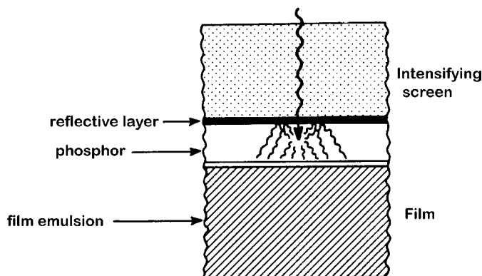
Fig. 15-24 Cross-section of a typical double-emulsion radiographic film overlain with an intensifying screen with a reflective layer and phosphor to increase the number of light photons reaching the film.
