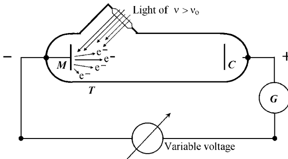
Fig. 2-11 Experimental arrangement for measuring photoelectric phenomena.
