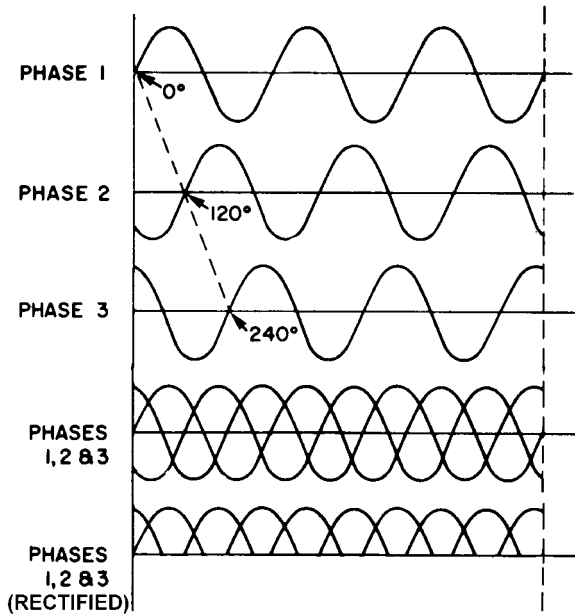
Fig. 15-13 Three-phase alternating current waveforms that are composited and rectified (the “ripple effect” in the rectified waveform can be further reduced to an almost steady output by increased phasing of voltage pulses).
