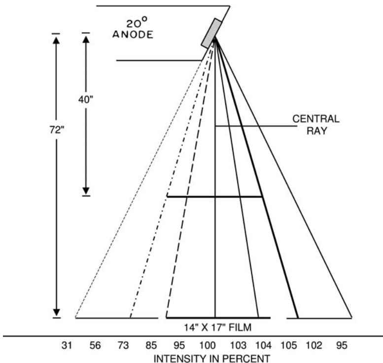
Fig. 15-7 Reduction in x-ray intensity due to the heel effect.
