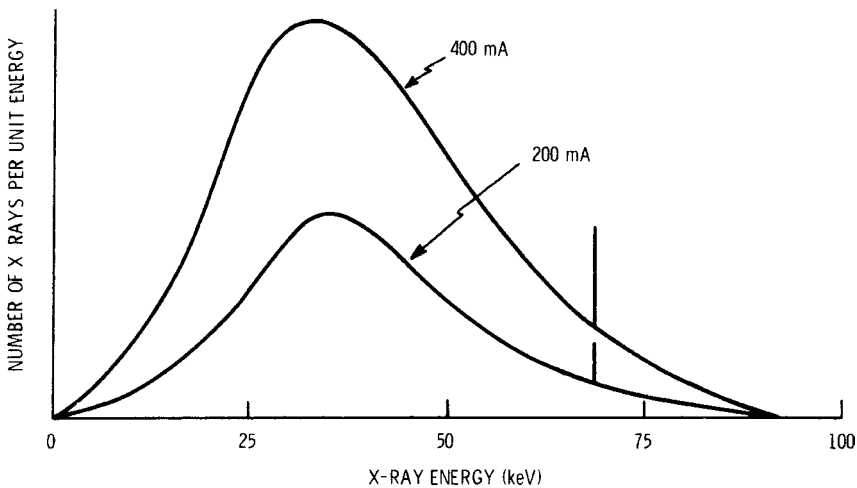
Fig. 15-12 Influence of mA s at constant kVp on the number of x-rays emitted.
