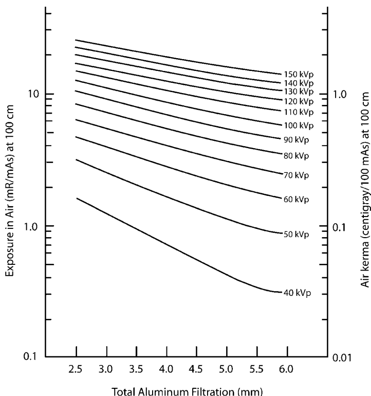
Fig. 15-29 Exposure rates in air, without backscatter, from typical diagnostic three-phase x-ray equipment for a target-skin distance of 100 cm; these values would be a factor of 1.7 lower for a single-phase high-voltage supply.
