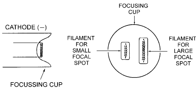
Fig. 15-6 Typical focusing cup arrangement with a double filament in the cathode of an x-ray tube.
