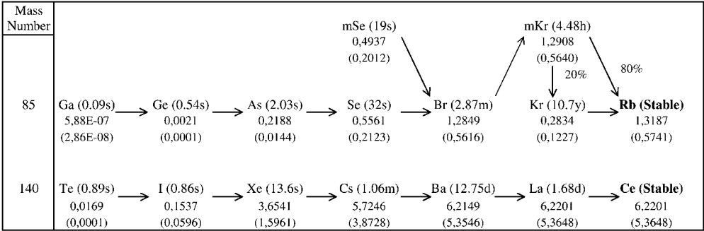
Fig. 5-21 Total fission product yields for each fission product mass number due to thermal fission of ^{235}\text{U} and ^{239}\text{Pu} .
