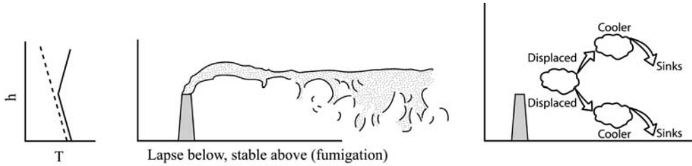
Fig. 10-6 Fumigation breakup of a trapped plume producing a zone of relatively high concentration between the ground and the bottom of the inversion layer, typically at H_e .
