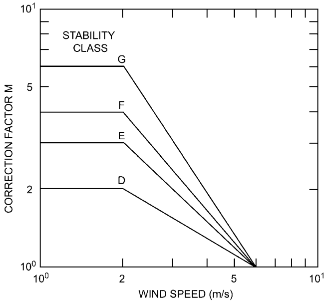
Fig. 10-8 Meander factor M for determining \Sigma_y for far-field dispersion downwind of buildings and obstacles.
