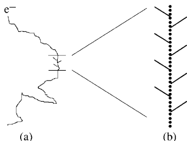
Fig. 7-5 (a) Range and ionization path of a beta particle in an absorbing medium; (b) amplified segment of ionization track showing delta ray tracks produced by ejected electrons.
