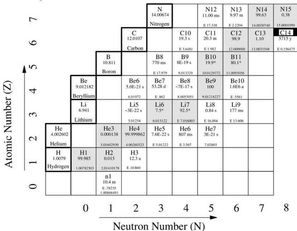
Fig. 1-1 Part of the chart of the nuclides. (Source: Chart of the nuclides, Nuclides and Isotopes , 15th edn, General Electric Co., 1996.)
