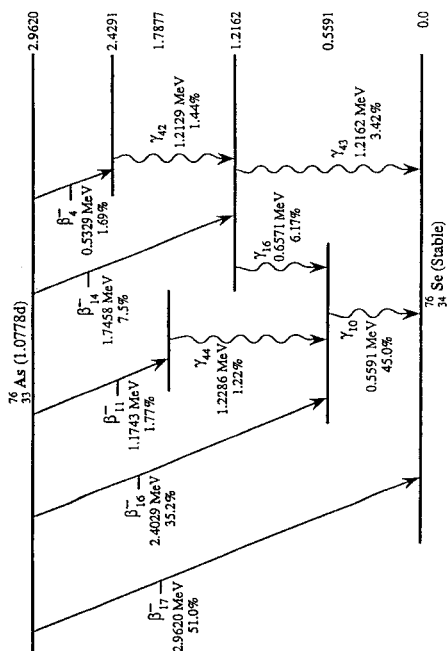
75 As(n,γ) (Mar. 15, 1995)
