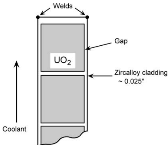
Fig. 5-19 \text{UO}_2 fuel pellet in zircalloy cladding.
