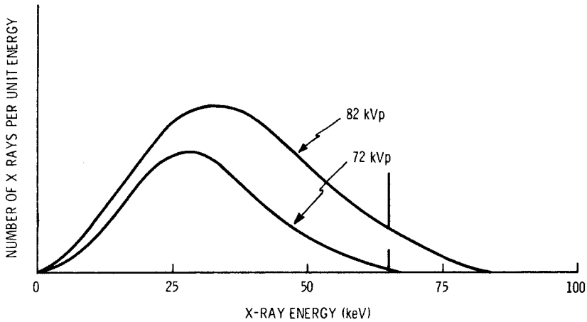
Fig. 15-11 Influence of x-ray tube voltage on the energy distribution of emitted x-rays in which an increase in kVp increases both the average and maximum energy of emitted x-rays.
