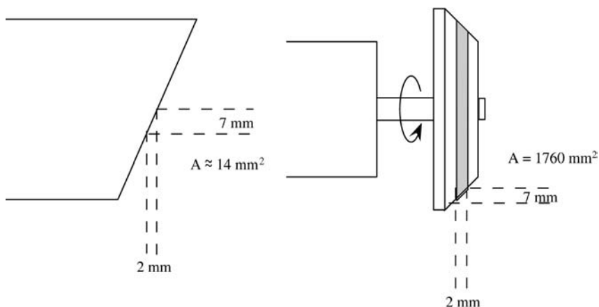
Fig. 15-8 Heat dissipation area of an x-ray tube with a stationary anode versus one with a rotating anode.
