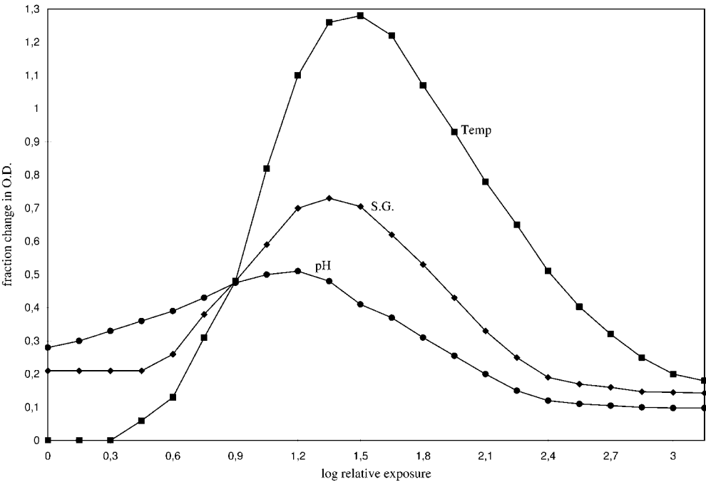
Fig. 15-28 Influences of changes in developer temperature, pH, and specific gravity (S.G.) on the characteristic curve for radiographic film (Kasza 1989).
