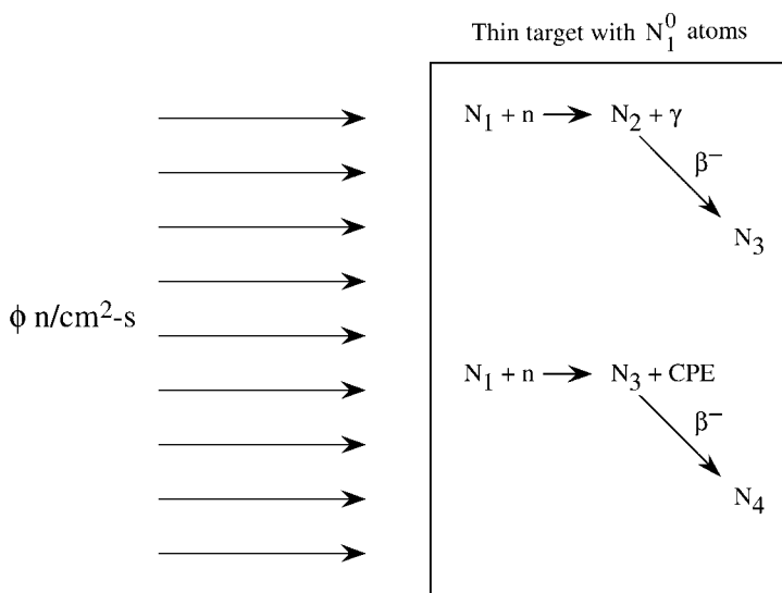
Fig. 4-18 Schematic of neutron irradiation of a thin (greatly amplified) target material to produce new atoms of a radioactive product.
