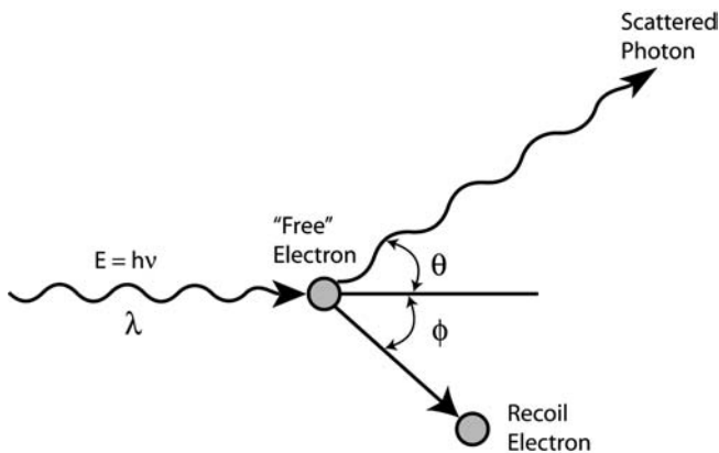
Fig. 2-14 Compton effect for x-ray scattering represented as a collision between an incident photon and a loosely bound or “free” electron producing a scattered photon of reduced energy (i.e., longer wavelength) and a recoiling electron.
