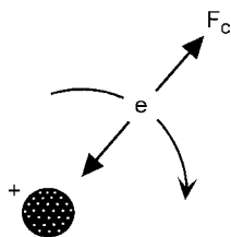
Fig. 2-24 Electron in a Bohr orbit experiences a coulombic force of attraction towards the nucleus that is counterbalanced by the centrifugal force due to its orbital motion.
