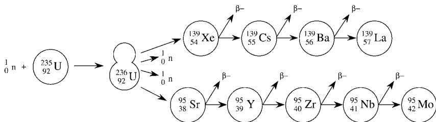
Fig. 5-2 Uranium-235 fission and the series of radioactive transformations by beta emission of the fission products to stable end products when mass numbers 95 and 139 are produced.
