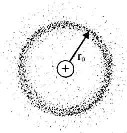
Wave-mechanical model of H
