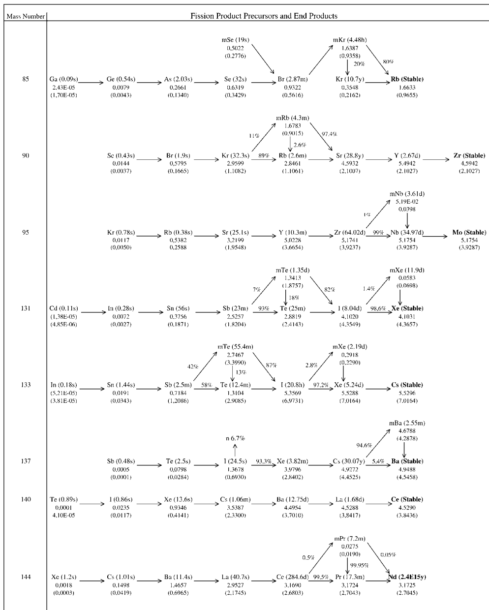
Fig. 11-9 Cumulative percent fission yields for fast neutrons in ^{235}\text{U} and ^{239}\text{Pu} for each isotope in selected mass chains.
