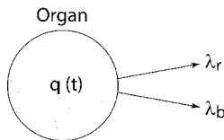
Fig. 9-1 Radionuclide consisting of N atoms with activity q(t) = \lambda N is assumed to be distributed uniformly in an organ mass from which radioactive atoms are cleared by both radioactive transformation ( \lambda_r ) and biological removal ( \lambda_b ).
