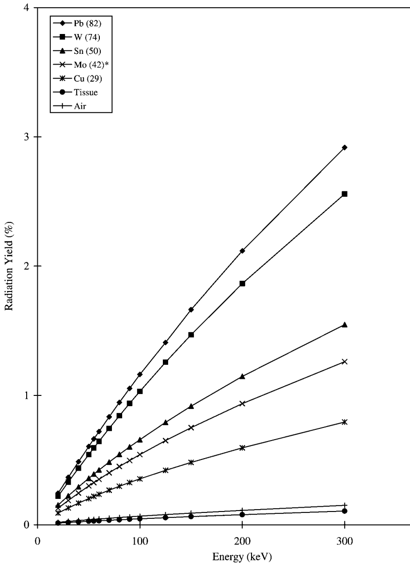
Fig. 15-4 Percent radiation yield for electrons of initial energy E on different absorbers.
