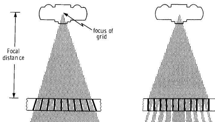
Fig. 15-23 Focused grid with grid strips angled to the path of x-ray photons and a linear grid with parallel strips resulting in some cutoff of the x-ray beam at the outer edge. (Adapted from Bushong (2004), with permission.)
