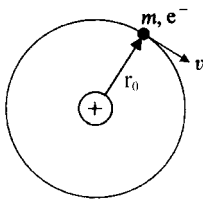
Bohr model of H
