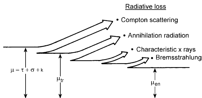
Fig. 7-18 Relationship of the photon attenuation coefficient \mu the energy transfer coefficient \mu_{\text{tr}} = \mu - \sigma_s , and the energy absorption coefficient \mu_{\text{en}} , and the radiative loss processes that propagate energy out of the absorbing medium.
