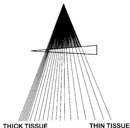
Fig. 15-15 Use of a wedge filter to shape an x-ray beam for radiography of nonuniform anatomy as may be encountered in a thoracic spine examination.
