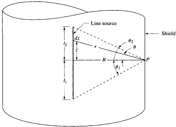
Figure 10.11 Isotropic line source imbedded in a cylindrical shield.
