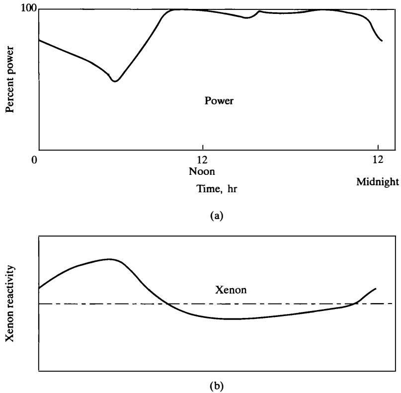
Figure 7.16 (a) Nominal weekday load of Consolidated Edison Company of New York; (b) the buildup and burnout of xenon in a reactor responding to this load.
