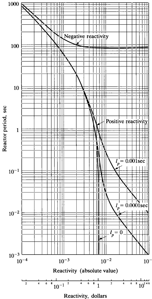
Figure 7.2 Reactor period as a function of positive and negative reactivity for a ^{235}\text{U} -fueled reactor.
