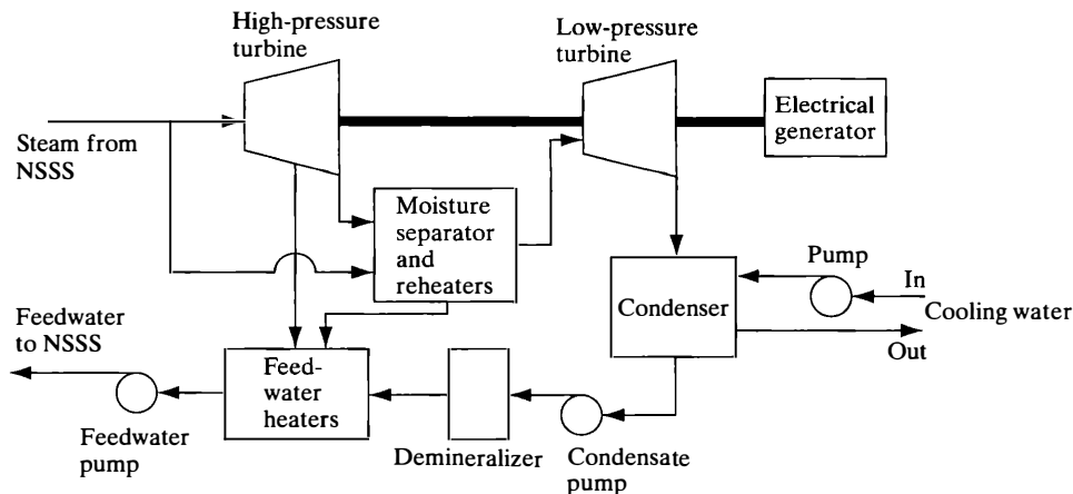
Figure 4.4 Simplified diagram of the power-producing side of a nuclear steam power plant.
