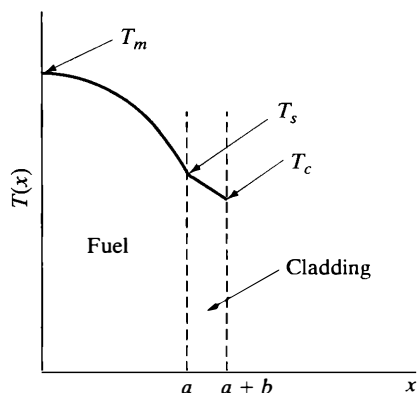
Figure 8.5 Temperature distribution across plate-type fuel element.
