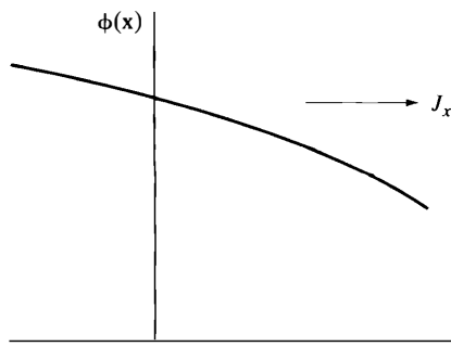
Figure 5.1 Neutron flux and current.
