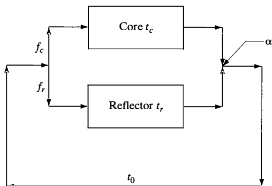
Figure 10.31 Schematic representation of coolant circuit showing flow split between core and reflector for Prob. 10.34.
