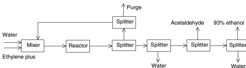
Figure 5.15. Ethanol process.
