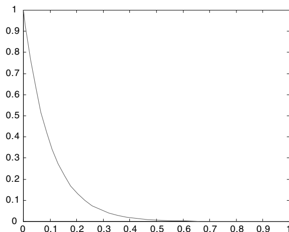
Figure 8.1. Solution to Eq. (8.16) using MATLAB.
