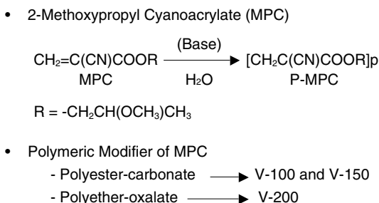
FIGURE 5.1 Chemistry of bioabsorbable tissue adhesives V-100, V-150 and V-200.
