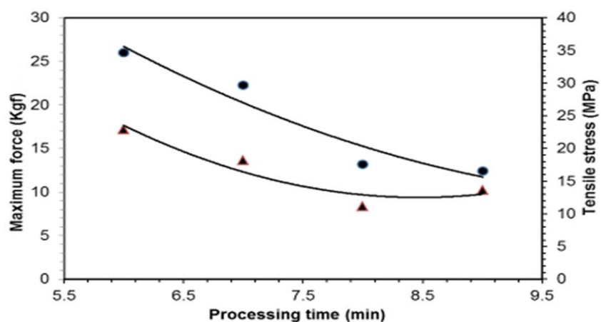
Fig. 2. Effect of different processing time on maximum force at yield point and tensile stress of the composite [●= maximum force; ▲= tensile stress]
