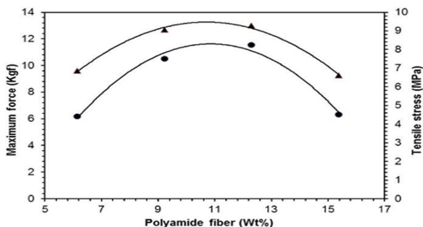
Fig. 4. Effect of different polyamide fiber contents on maximum force at yield point and tensile stress of the composite [●= maximum force; ▲= tensile stress]
